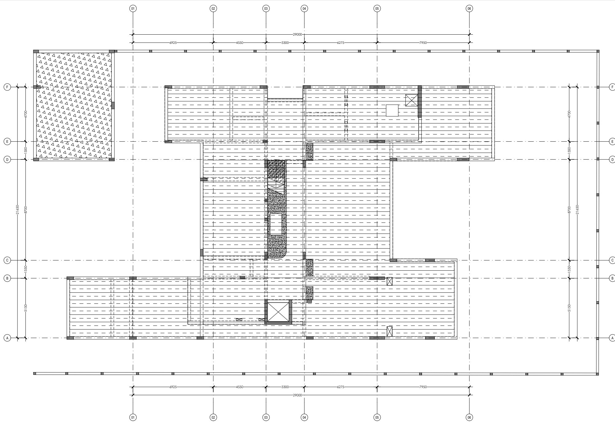
GROUND FLOOR LOADING PLAN SCALE: 1:250
